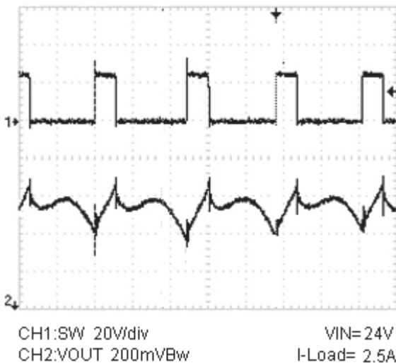
SW vs. Output Waveform
