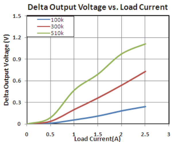
Figure 1. Delta Output Voltage vs. Load Current
