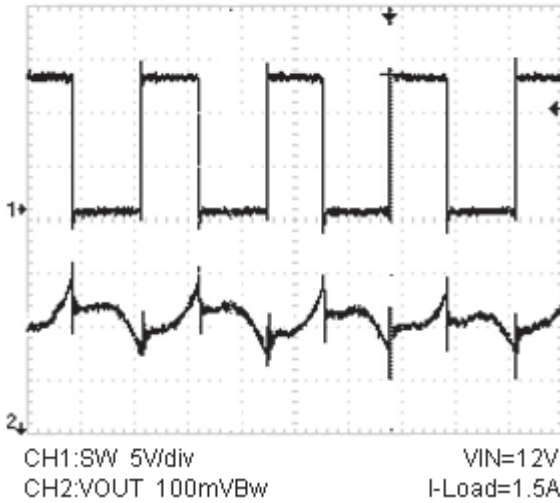
SW vs. Output Waveform
