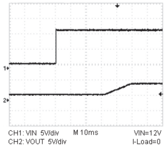
Start-up Waveform
